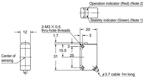
CX-31A CX-31B CX-39A CX-39B Sensor
